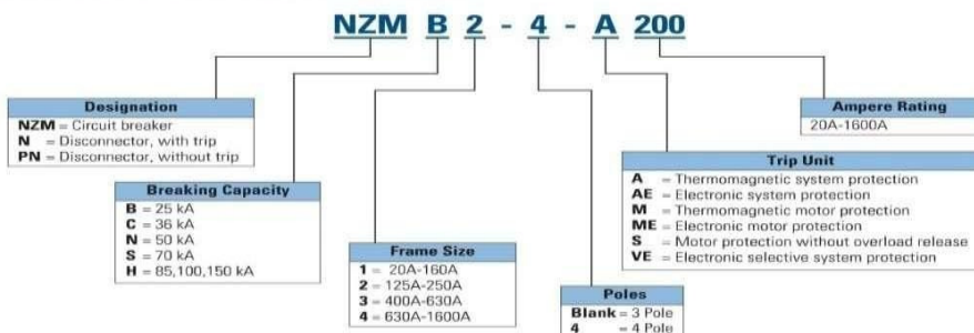
NZM Series Molded Case Circuit Breaker
